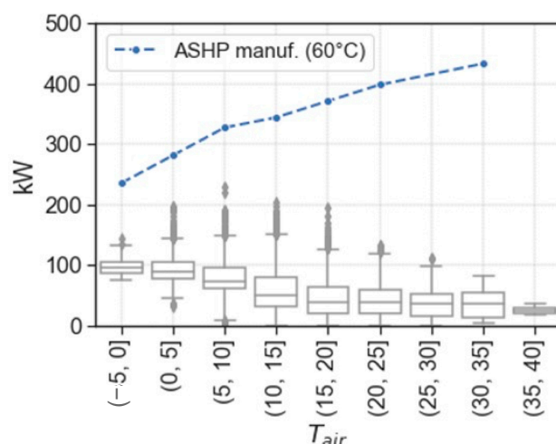
Figure 9. Monovalent ASHP system: Hourly heat load ( \text{kW}_{\text{th}} ) by bins of outdoor temperature of 5^\circ\text{C} , in relation to the HP capacity (July 2019 to June 2020). The heat load is represented by boxplots, with 50% of the hourly heat load within the box (median \pm 25\% ), 80% within the upper and lower marker, and the 10% min and max outliers represented by dots.
