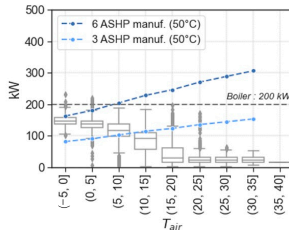
Figure 14. Hybrid ASHP system: Hourly heat load (kW th by bins of outdoor temperature of 5 °C), in relation with the HP and boiler capacity (July 2018 to June 2019). The heat load is represented by boxplots, with 50% of the hourly heat load within the box (median +/−25%), 80% within the upper and lower marker, and the 10% min and max outliers represented by dots.
