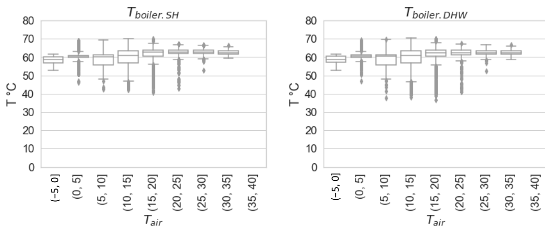
Figure A9. Hybrid system, boiler production temperature (by bins of outdoor temperature of 5 °C), SH mode, and DHW mode. The temperature spread is represented by boxplots, with 50% of the hourly heat load within the box (median +/−25%), 80% within the upper and lower marker, and the 10% min and max outliers represented by dots.
