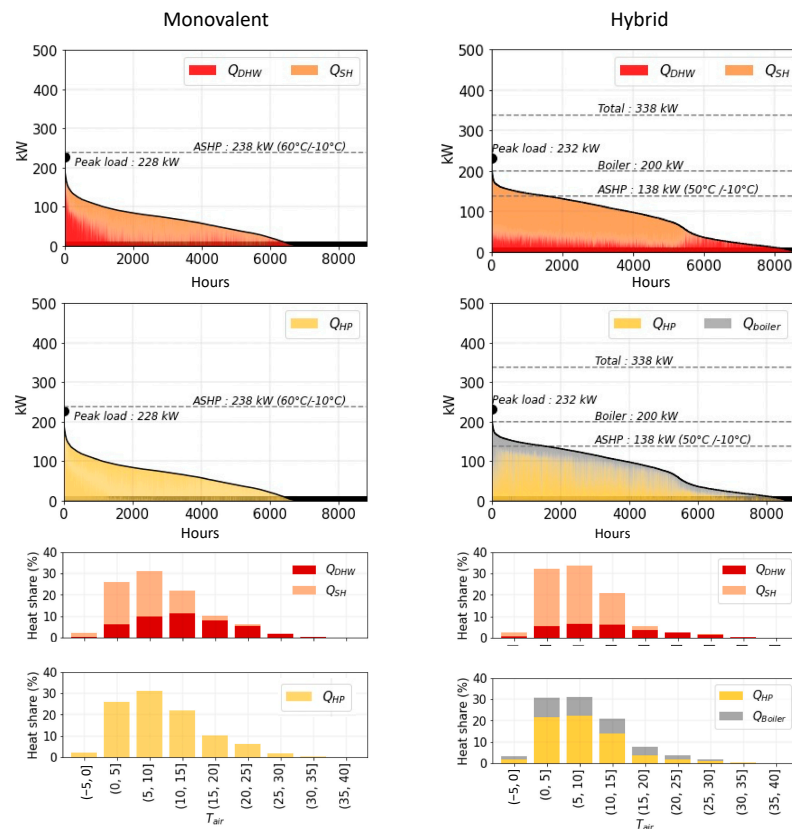
Figure A7. Monovalent and hybrid system; (Top) Sorted hourly heat production, decomposed in DHW and SH, as well as in HP and boiler, with related design capacities ( \text{kW}_{\text{th}} ); (Bottom) Heat share (by bins of outdoor temperature of 5^\circ\text{C} ), segmented in SH and DHW, as well as in HP and boiler.
