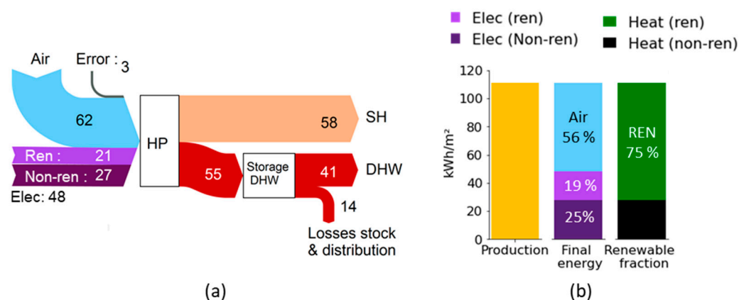
Figure 6. (a) Sankey diagram of the monovalent ASHP system in kWh/m²/yr. (b) Heat production, decomposed by source and renewable/non-renewable energy fraction. Second year of operation (1 July 2019 to 30 June 2020) in kWh/m²/yr.
