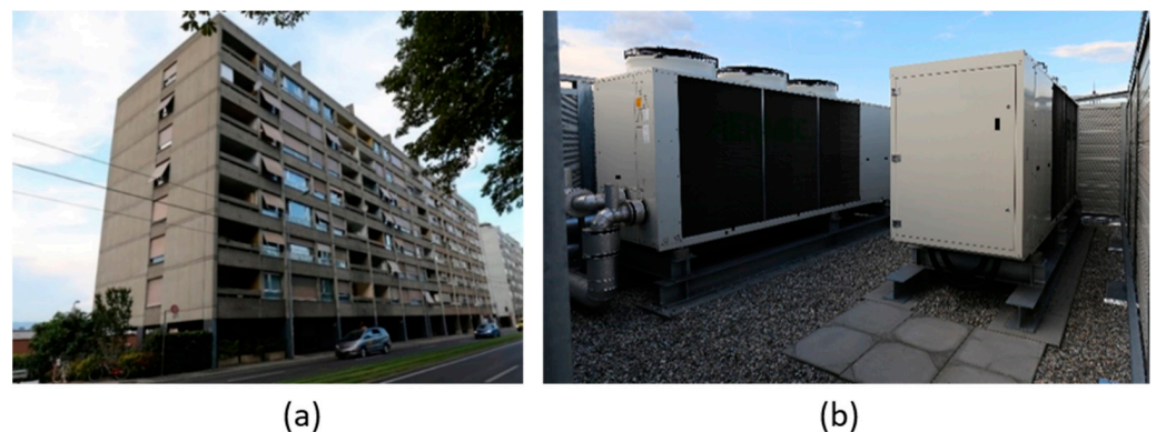
Figure 2. Monovalent ASHP system. (a) non-retrofitted MFB and (b) industrial ASHP on the roof with sound-proofing wall panels.
