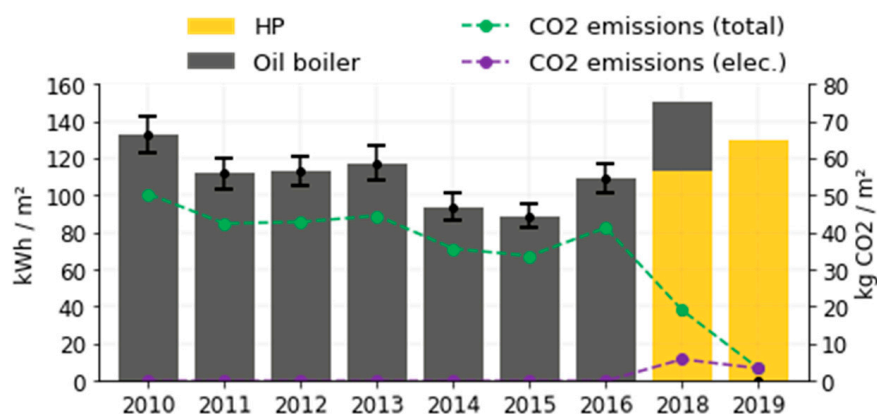
Figure 7. Monovalent ASHP system: evolution of the heat production (normalized to standard weather) in kWh th /m²/yr and CO 2eq emissions in kgCO 2eq /m²/yr, over the 2010–2019 period. Each year runs from July to June of the next year (e.g., 2019 = 1st July 2019 to 30th June 2020). The error bars represent the heat production uncertainty due to the boiler efficiency estimated at 70% ± 5%.
