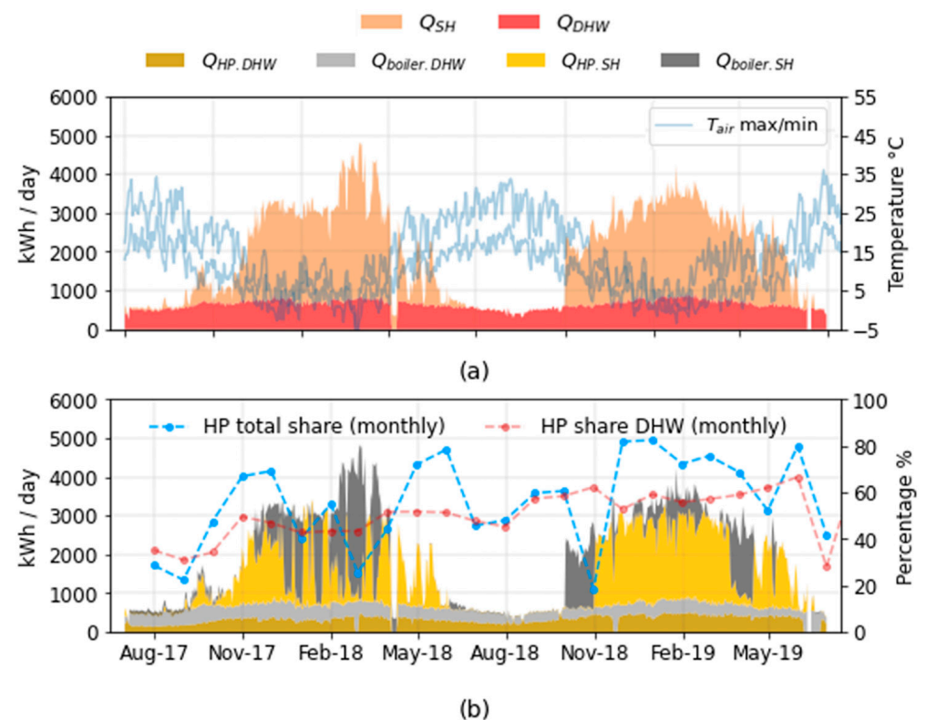
Figure 13. Hybrid ASHP system: (a) Daily SH and DHW production ( kWh_{th}/day ), as well as minimum/maximum outdoor temperature and (b) Daily HP and boiler production ( kWh_{th}/day ), segmented between SH and DHW (left axis), as well as ASHP share (right axis), over two years of operation (July 2017–June 2019).
